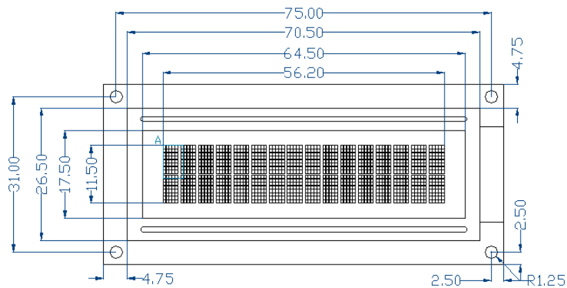
Figure 17: LK162-12 Screen Drawing
