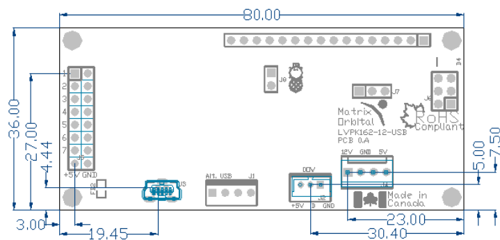
Figure 19: LK162-12-USB Dimensional Drawing
