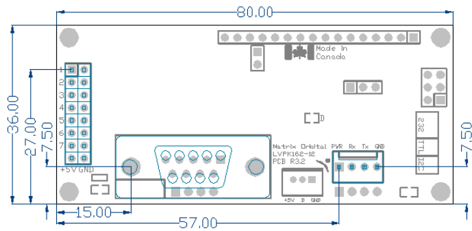
Figure 18: LK162-12 Dimensional Drawing
